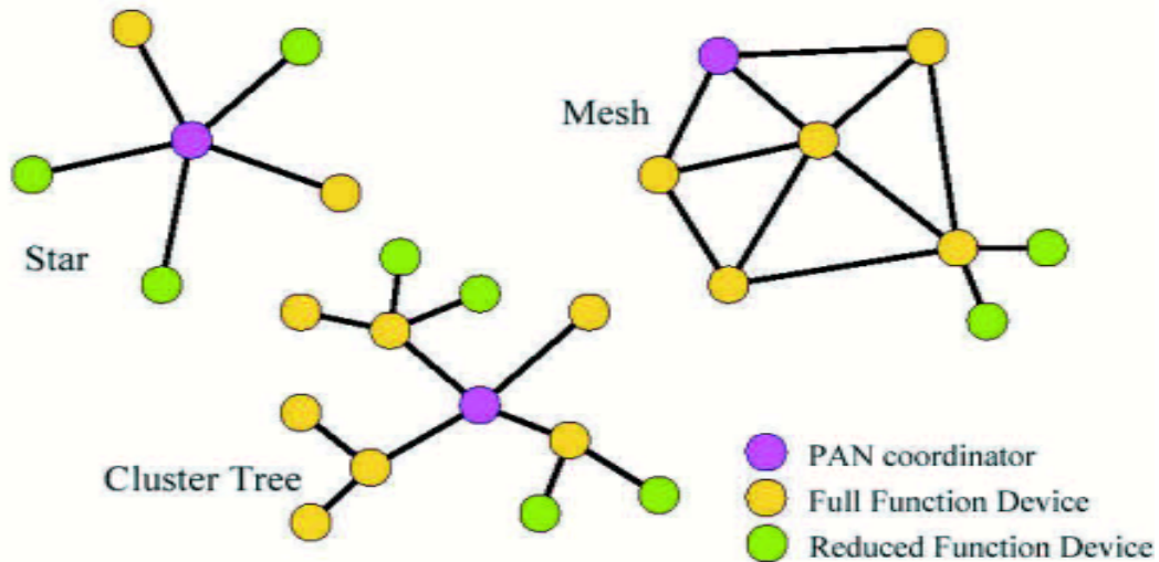
Fig.2: Topology Models.
