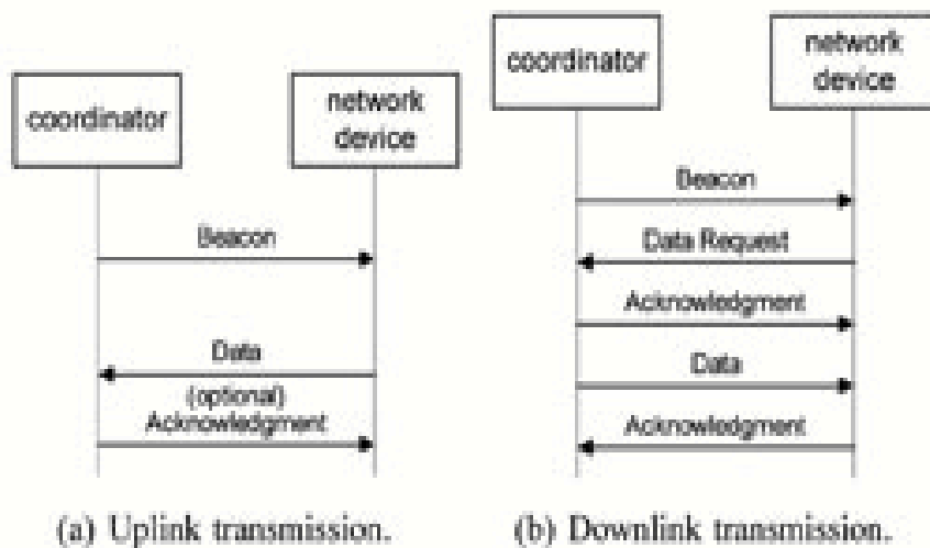
Fig. 3: Data transfer in 802.15.4 PAN in beacon enabled mode.
