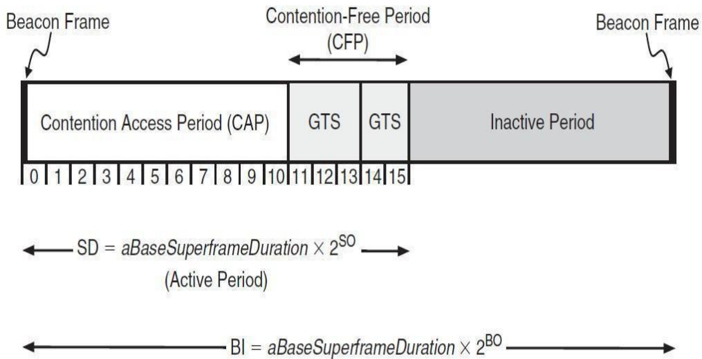
Fig. 4: Super frame Structure.
