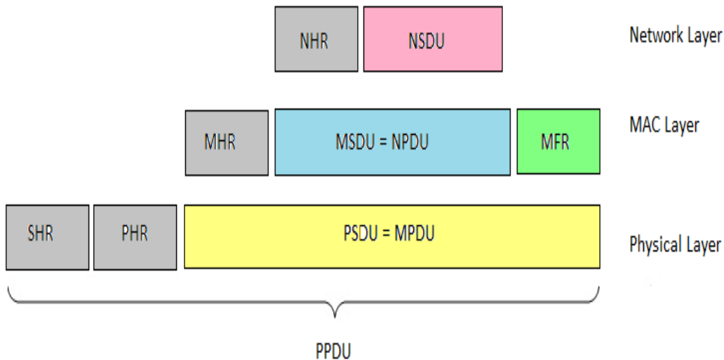
Fig. 1: Structure of the IEEE 802.15.4.
